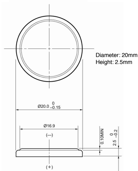
Dimension Drawing
