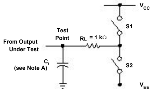
LOAD CIRCUIT
