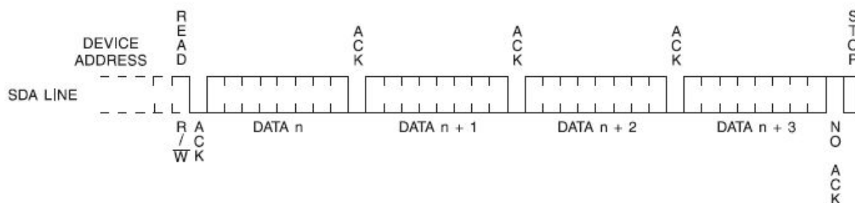
Figure 9. Sequential Read
