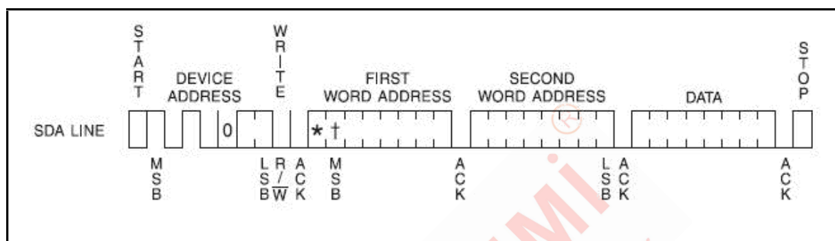
Figure 5. Byte Write
