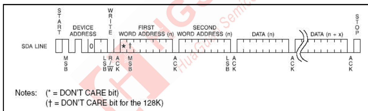
Figure 6. Page Write
