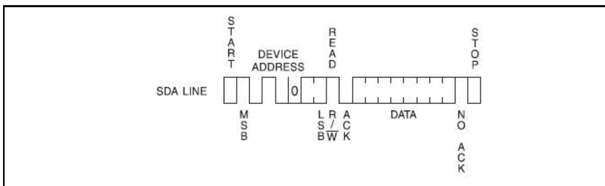
Figure 7. Current Address Read
