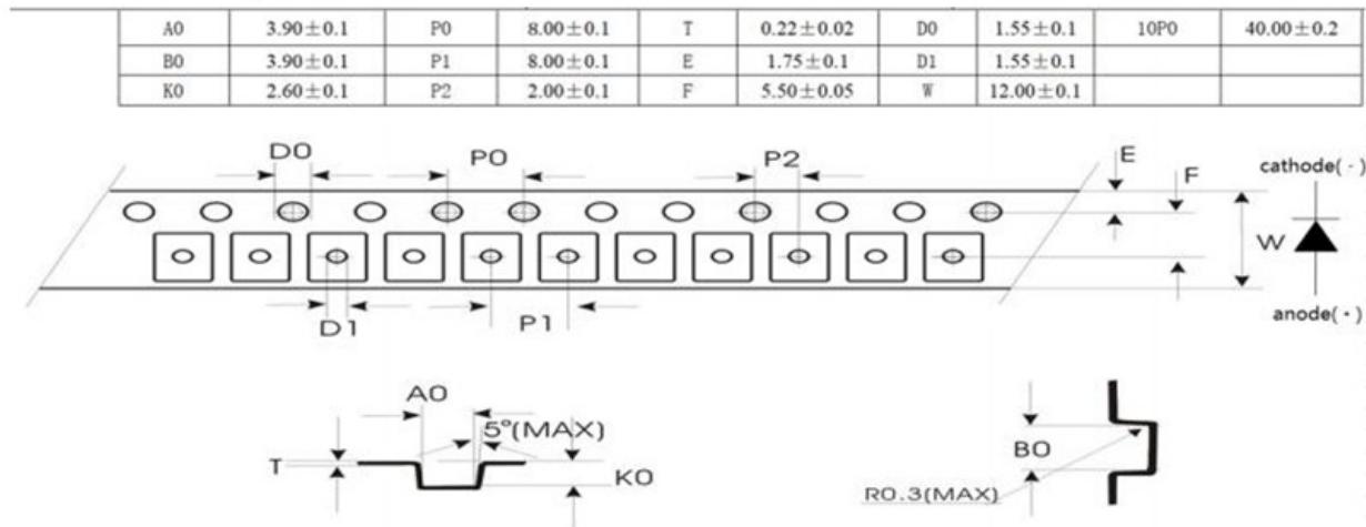
Dimension of Tape 载带规格
