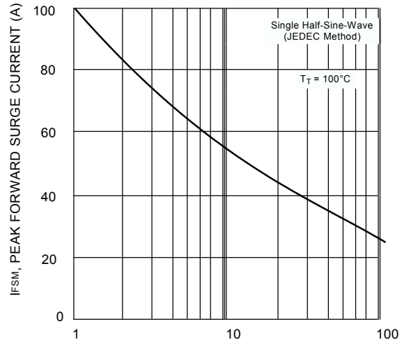
Fig. 4 Max Non-Repetitive Peak Fwd Surge Current
