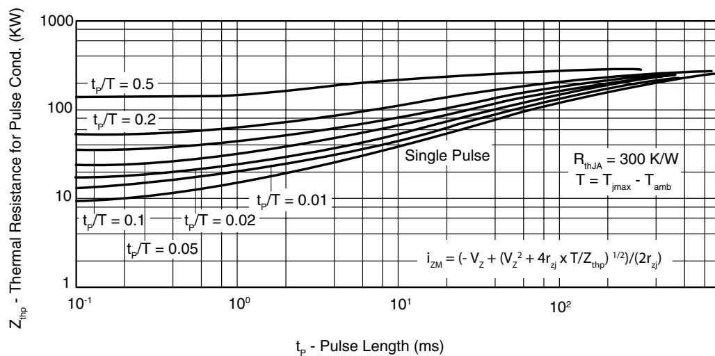
Figure 10. Thermal Response
