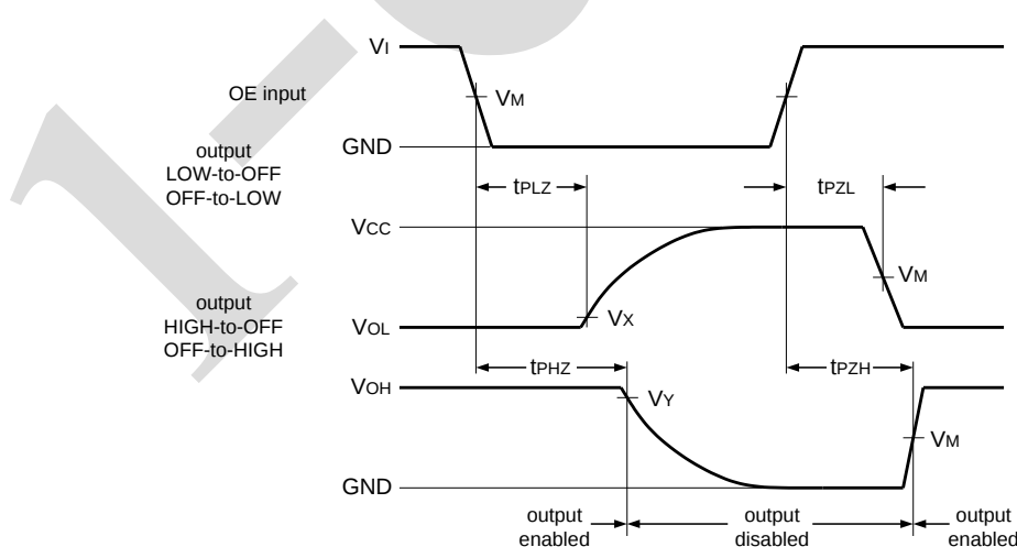
Figure 6. 3-state enable and disable times
