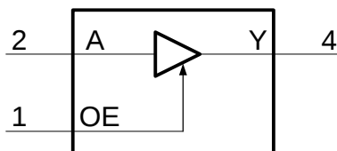
Figure 1. Logic symbol
