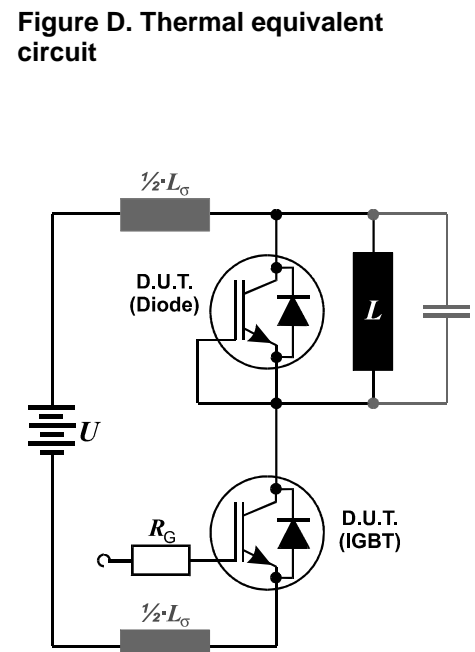
Leakage inductance L_\sigma=180\text{nH} , and stray capacity C_\sigma=40\text{pF} .
