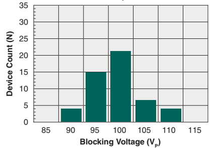
Typical Blocking Voltage Distribution (N=50, I F =1mA)
