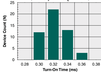
Typical Turn-On Time (N=50, I F =2mA, I L =100mA)
