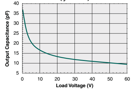
Output Capacitance vs. Load Voltage ( I_F=0.5mA )
