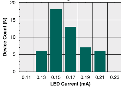
Typical I F for Switch Operation (N=50, I L =150mA)
