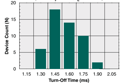
Typical Turn-Off Time (N=50, I F =2mA, I L =100mA)
