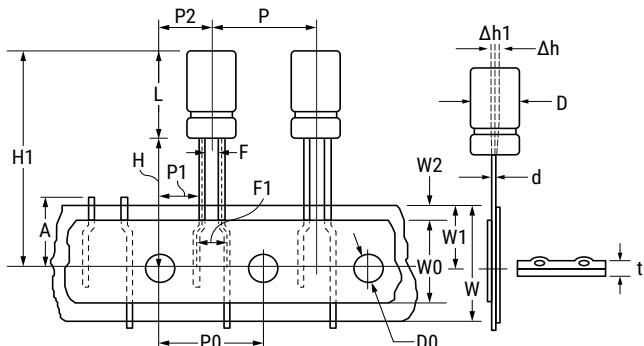
Fig. 3 (Diameter for \Phi 6 to \Phi 8 ) 6 – 8 mm EA
