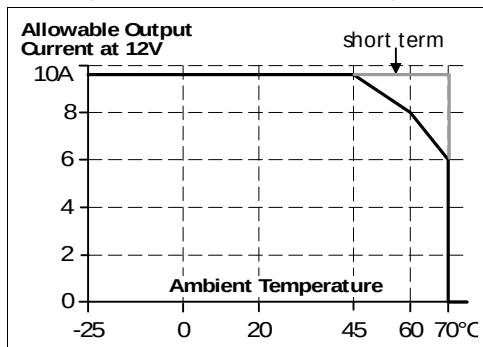
Fig. 14-1 Output current vs. ambient temp. (Inom 8A; Iout with PowerBoost = 9.6A)
