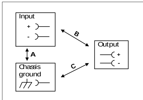
Fig. 17-1 Dielectric strength
