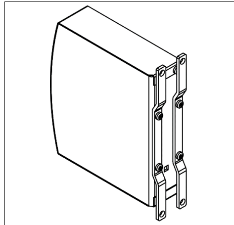
Fig. 21-2 ZM1.WALL attached to PSU*)
