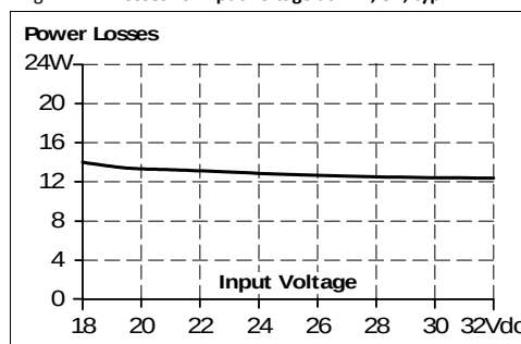
Fig. 7-4 Losses vs. input voltage at 12V, 8A, typ.
