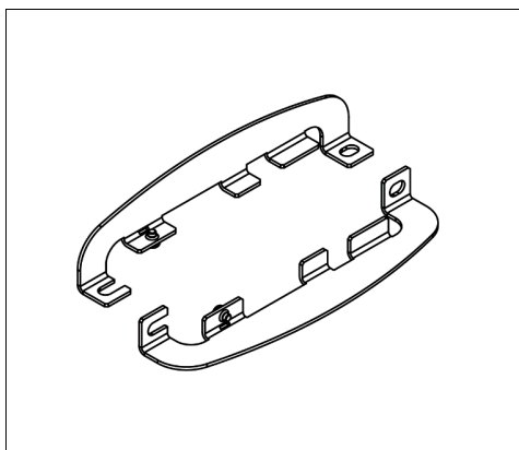
Fig. 21-1 ZM10.Wall Wall mounting bracket*)
