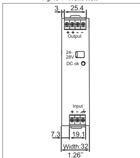
Fig. 19-1 Front view
