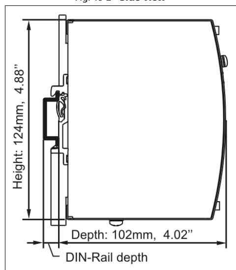
Fig. 19-2 Side view
