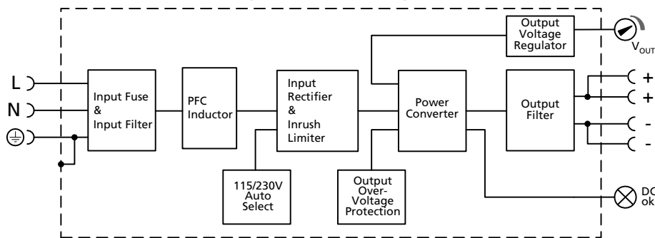
Fig. 10-1 Functional diagram
