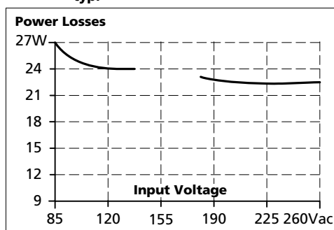
Fig. 8-4 Losses vs. input voltage at 48V, 5A, typ.
