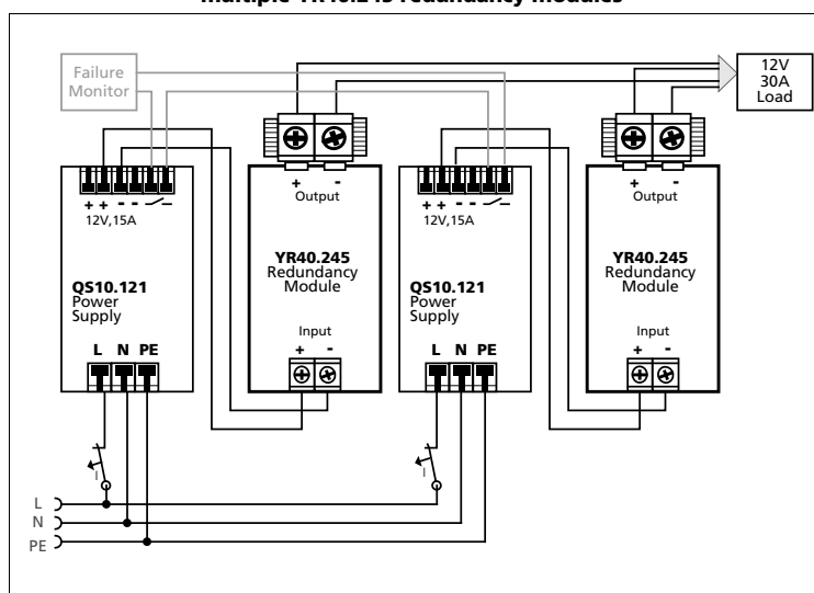
Fig. 21-2 Typical N+1 or 1+1 Redundant configuration for 15A with multiple YR40.245 redundancy modules
