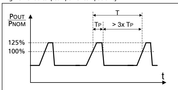
Fig. 25-Periodical peak power compatibility.
