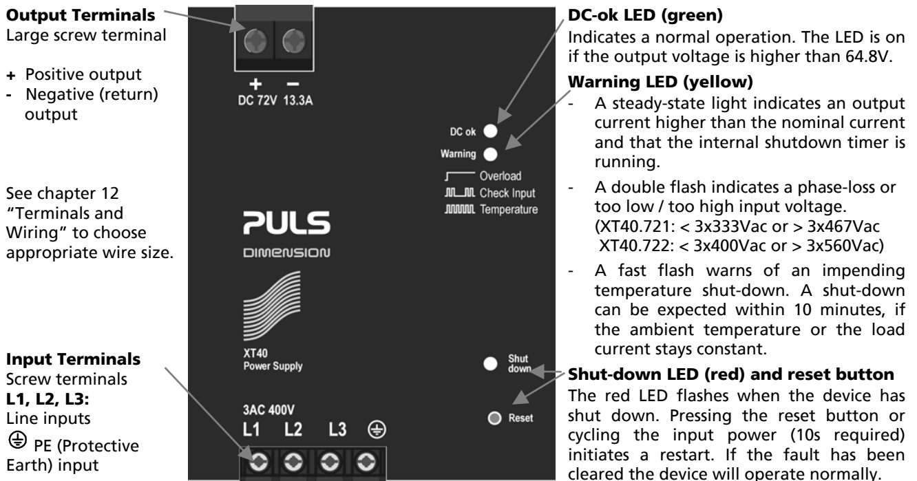
Fig. 11-1 Front side of XT40.721
