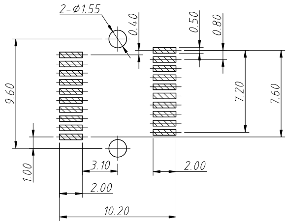
Detail A(2:1)
