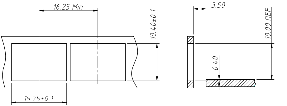
Bezel Recommended Bezel Thickness 0.8-2.6mm Bezel Opening Below Top Of PCB
