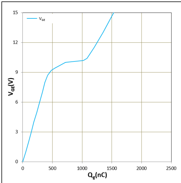
Figure 15. Gate charge
