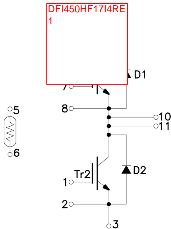
Figure 1. Out drawing & circuit diagram for DFI450HF17I4RE1
