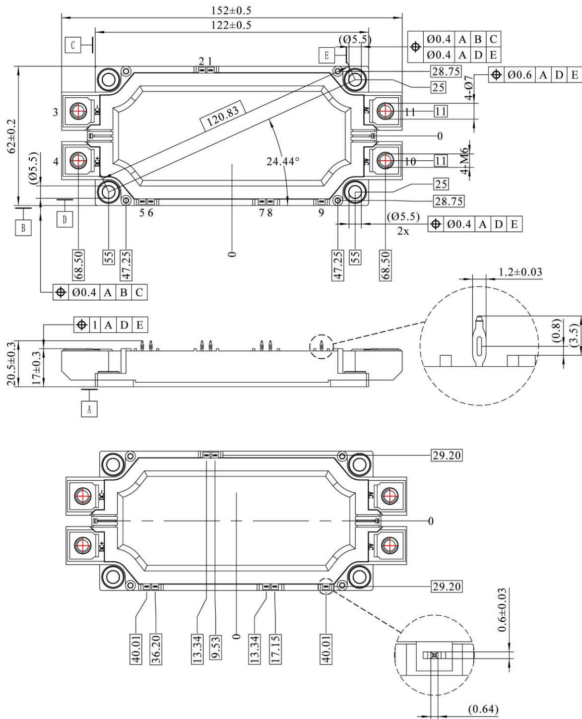
Figure 2. Pin configuration
