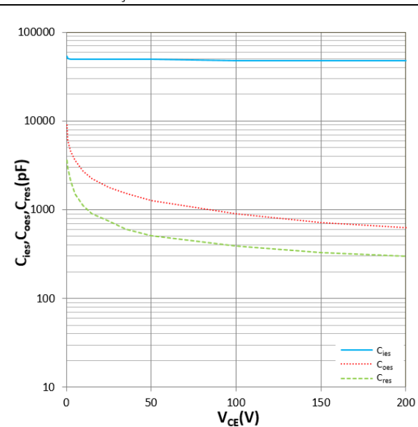
Figure 16. C_{ies} , C_{oes} , C_{res} vs V_{CE} T_J=25^{\circ}C , f=1MHz
