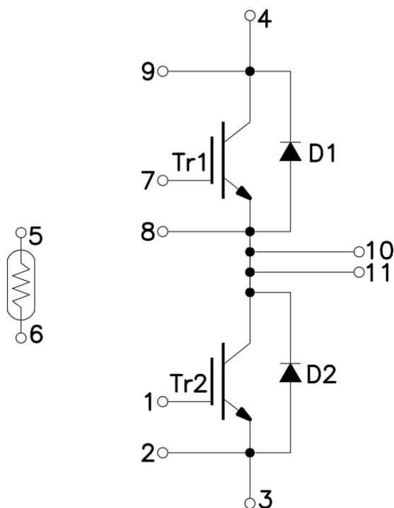
Figure 1. Out drawing & circuit diagram for DFI600HF17I4RE1P
