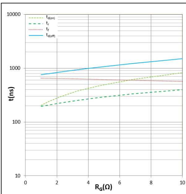
Figure 13. Switching time vs R_G (Typ) V_{CC}=900V , V_{GE}=+15V/-8V , I_C=600A T_J=150^{\circ}C , Inductive Load
