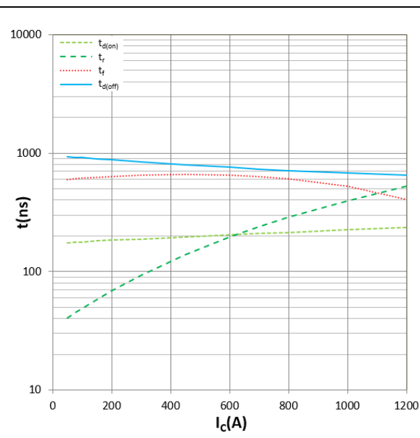
Figure 14. Switching time vs I_C (Typ) V_{CC}=900V , V_{GE}=+15V/-8V , R_G=1.0\Omega T_J=150^{\circ}C , Inductive Load
