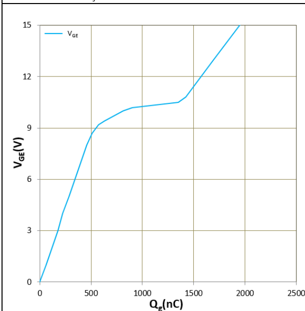
Figure 15. Gate charge
