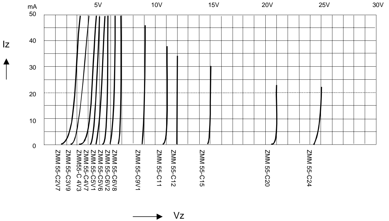
FIG.1- BREAKDOWN CHARACTERISTICS
