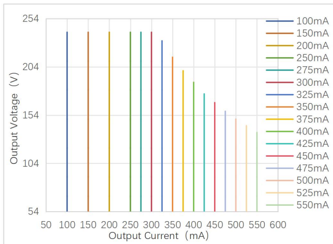
Operating Window
