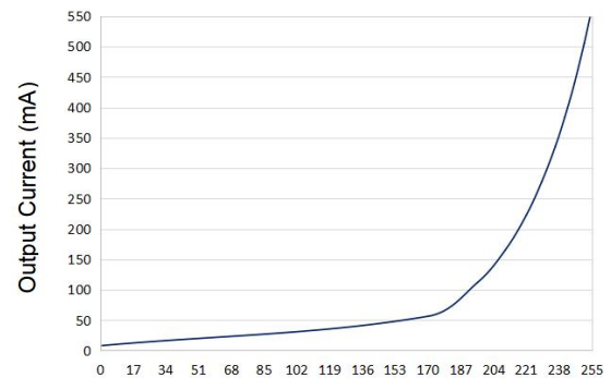
Logarithmic dimming
