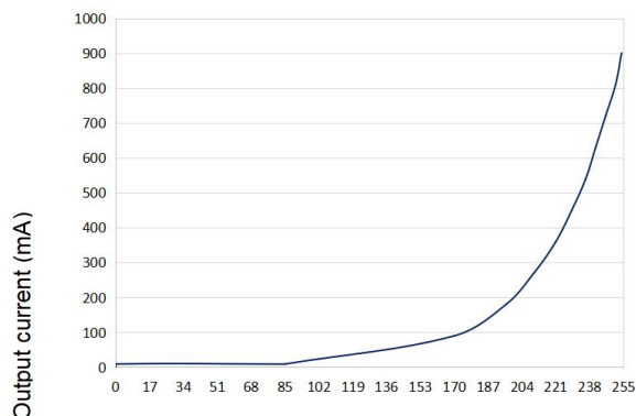
Logarithmic dimming
