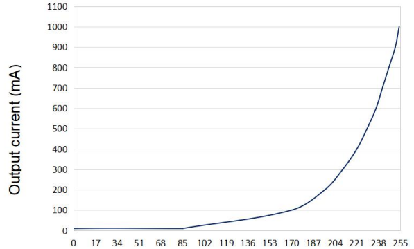
Logarithmic dimming
