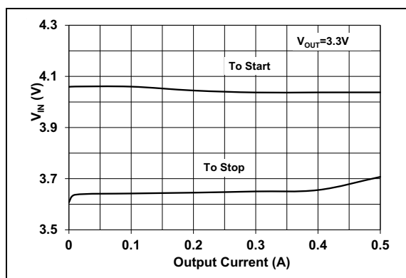
FIGURE 2-23: Minimum Input Voltage vs. Output Current.
