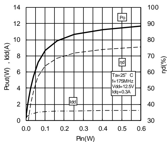
Pin-Po CHARACTERISTICS
