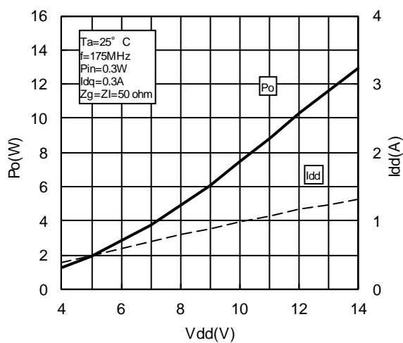
Vdd-Po CHARACTERISTICS
