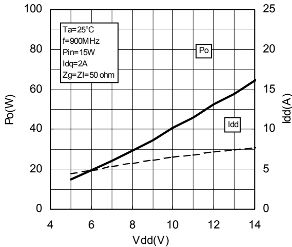
Vdd-Po CHARACTERISTICS
