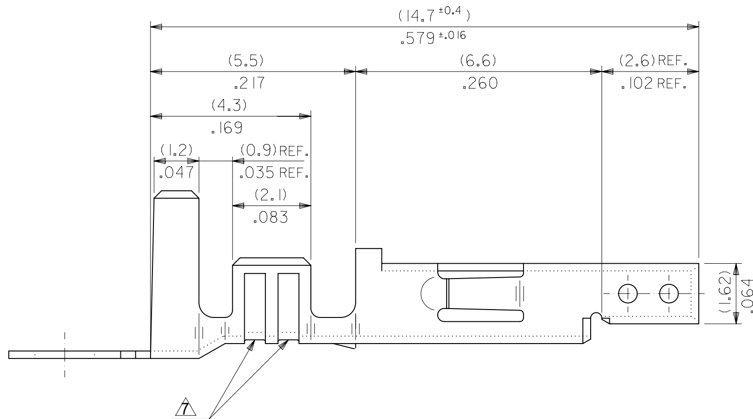
#18-24 TERMINAL SHOWN
