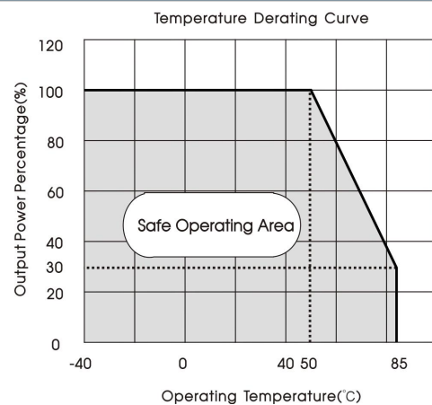
Fig.2 K78U24-300R3(L) (Vin ≥ 60V)
