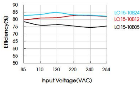
Efficiency Vs Input Voltage (Full Load)
