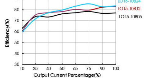
Efficiency Vs Output Load (Vin=230VAC)
