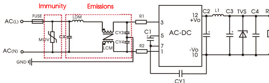
Recommended circuit 4
