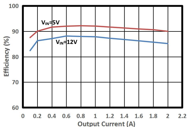
Figure 1. Efficiency vs. Load Current ( V_{OUT}=3.3\text{V} , f_{sw}=500\text{kHz} )
