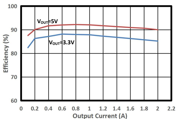
Efficiency vs. Output Current ( V_{\text{IN}}=12\text{V} , f_{\text{sw}}=500\text{kHz} )
