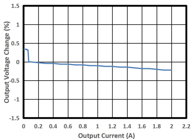
Figure 6. Load Regulation ( V_{OUT}=5\text{V} )
