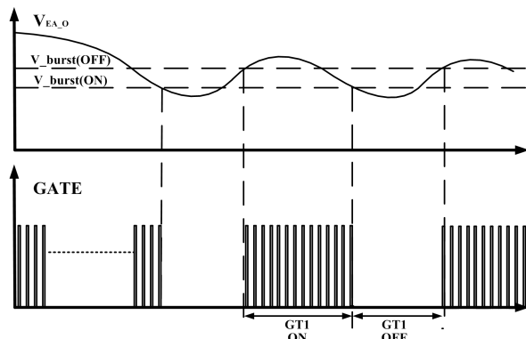
Figure 3 Light Load burst Mode
