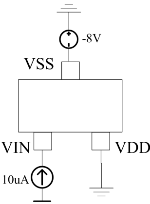
Fig. 2 Leakage Source Breakdown Volt Test Circuit
