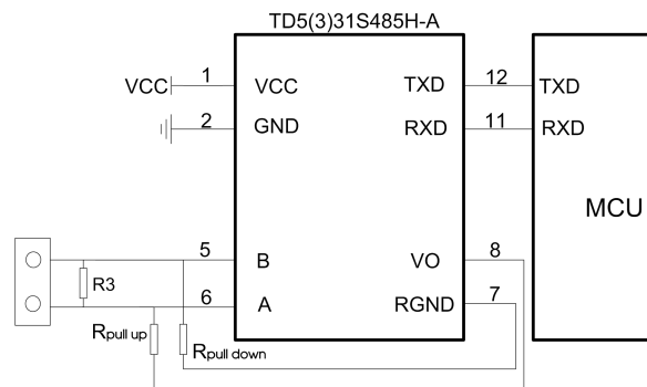
Fig. 1: Typical application
