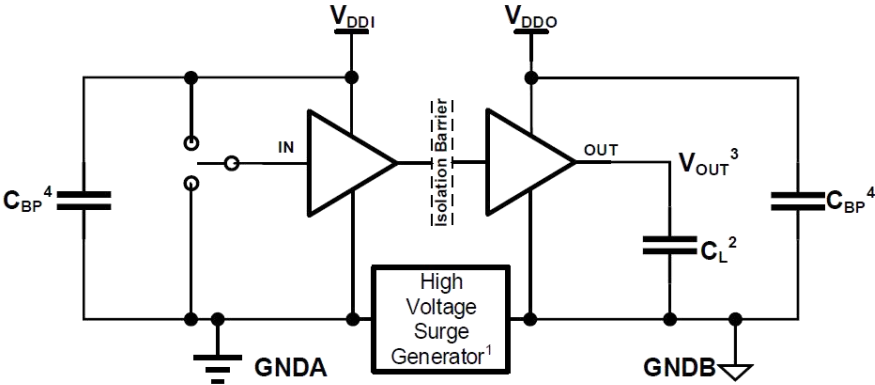
Figure 9. CMTI Test Circuit
