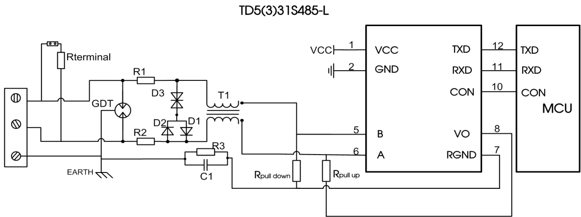
Fig. 2: Recommended protection circuit
