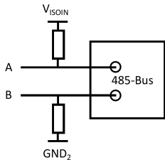
Figure13. Typical connection of pull-up and pull-down
