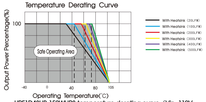
URF1D48HB-150WHR3 temperature derating curve (Vin=110V)
