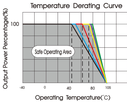
URF1D05HB-150WHR3 temperature derating curve (Vin=110V)
