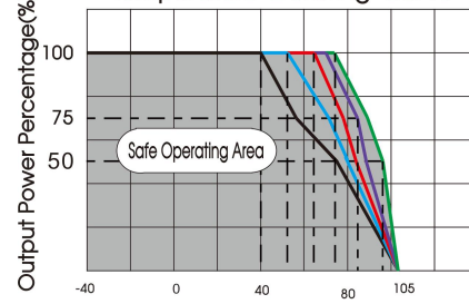
URF1D05QB-100WHR3 temperature derating curve (Vin=110V)
