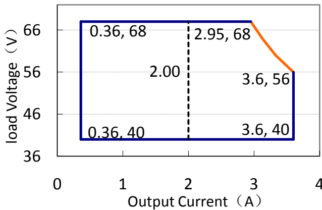
Output Current Vs Voltage Curve
