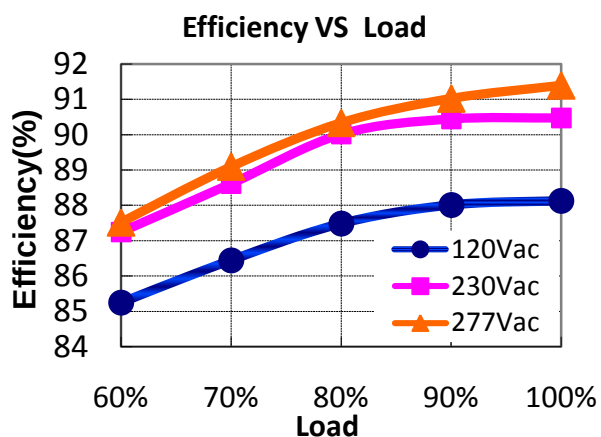
MTP-200X038( I_o=6.25A )
