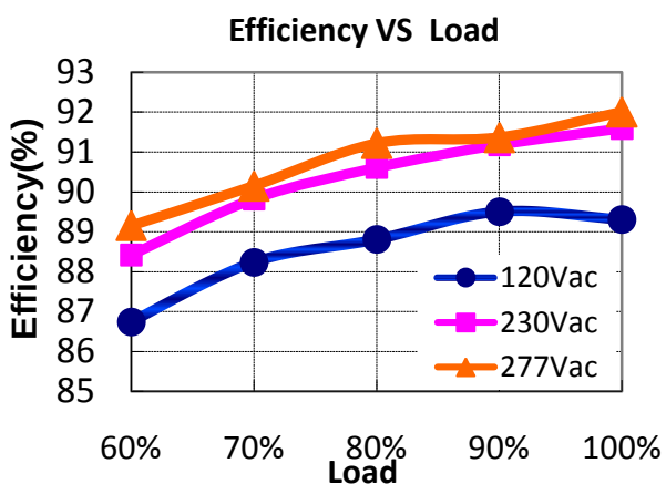
MTP-200X054( I_o=4.80A )
