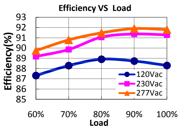
MTP-200X054( I_o=3.70A )
