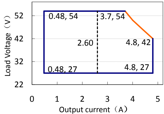
Output Current Vs Voltage Curve
