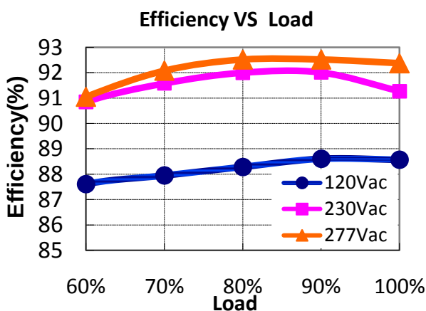
MTP-200X054( I_o=3.70A )
