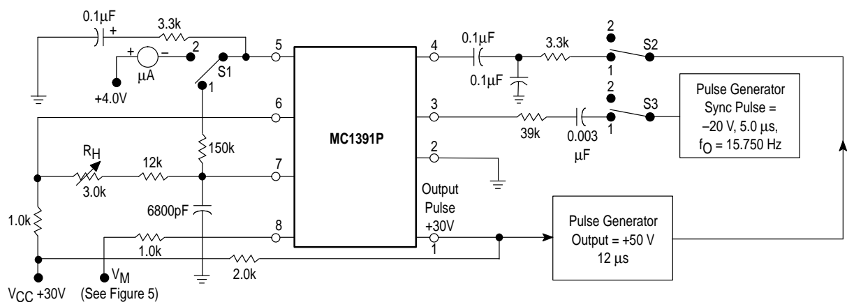
Figure 2. Test Circuit
