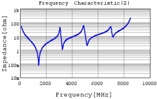
GQM2195C2E300GB12 |Z| DC0V, 25degC
