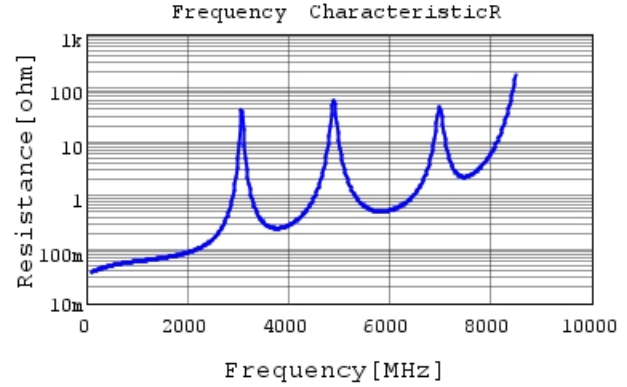
GQM2195C2E300GB12 R DC0V, 25degC
