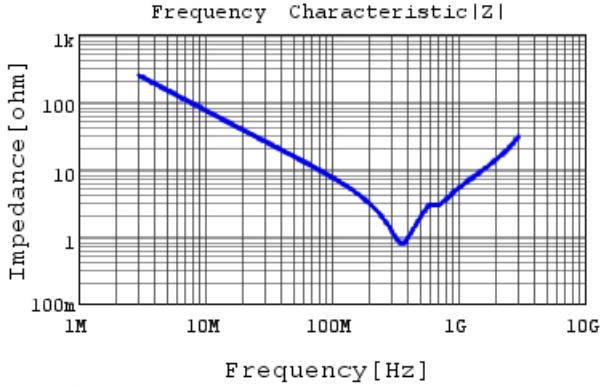
GR442QR73D221KW01 |Z| DCOV, 25degC
