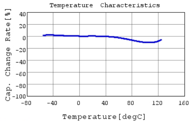
GR442QR73D221KW01 C-Temp. capchange, DCOV, 1
