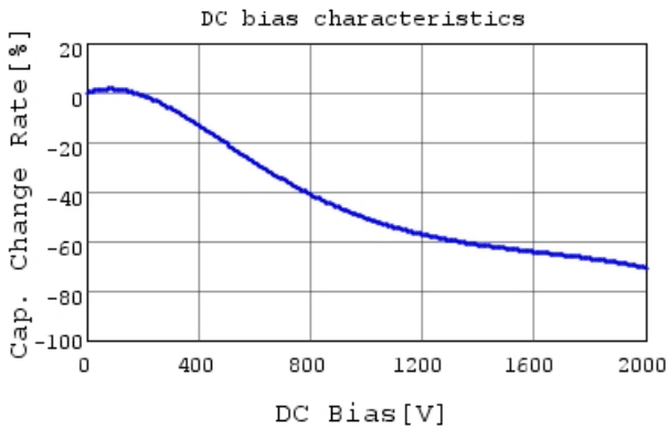
GR442QR73D221KW01 C-DC bias capchange, 25.0c
