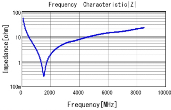
■ GRM1555C1H300JA01 |Z| DCOV, 25degC
