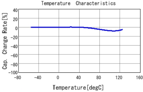
GRM21BR72A103KA01 C-Temp. capchange, DC0.0V, AC1.C
