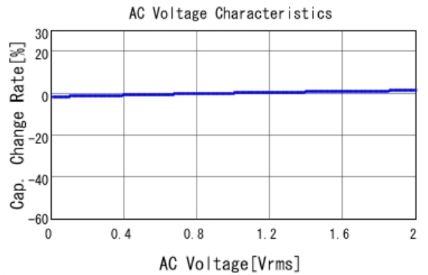
GRM21BR72A103KA01 C-AC Voltage capchange, DCOV, 25
