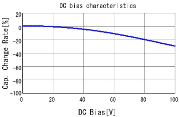
GRM21BR72A103KA01 C-DC bias capchange, 25.0degC, A
