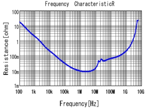
■ GRM31MR71H474KA01 R DCOV, 25degC
