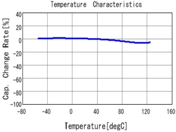
■ GRM31MR71H474KA01 C-Temp. capchange, DC0.0V, AC1.0V rm
