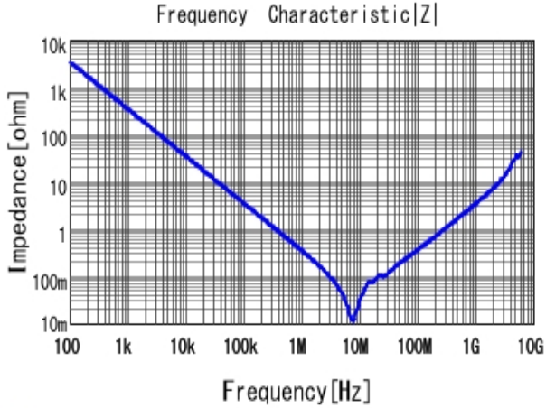
■ GRM31MR71H474KA01 |Z| DCOV, 25degC
