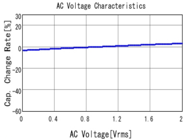
■ GRM31MR71H474KA01 C-AC Voltage capchange, DCOV, 25.0d
