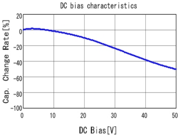
■ GRM31MR71H474KA01 C-DC bias capchange, 25.0degC, AC1.
