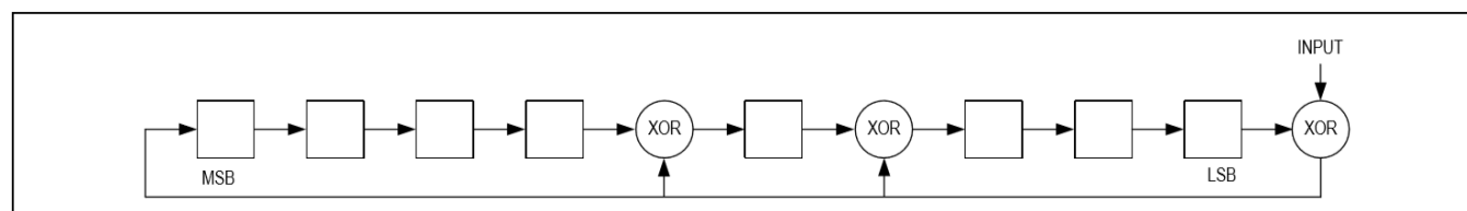
Figure 9. CRC Generator
