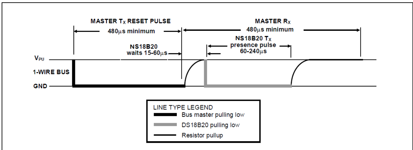
Figure 13. Initialization Timing
