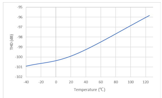
Figure 5.14 Total Harmonic Distortion vs Temperature
