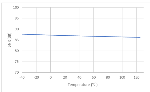
Figure 5.11 Signal-to-Noise Ratio vs Temperature
